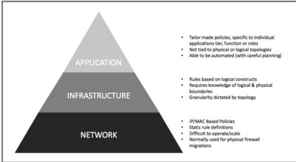
Figure 1 - Micro-segmentation Methodologies
