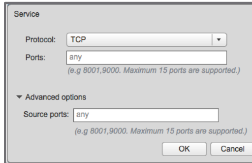
Figure 17 - Source/Destination: Protocols
