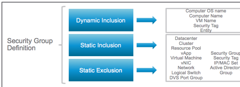
Figure 3 - Security Groups Definition
