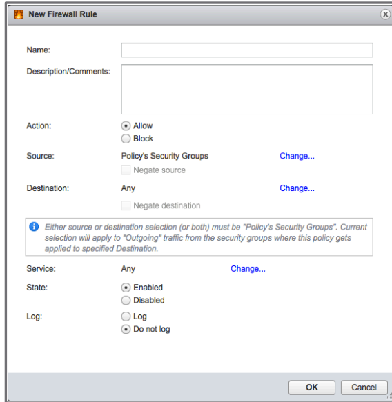
Figure 9 - Service Composer - New Firewall Rule
