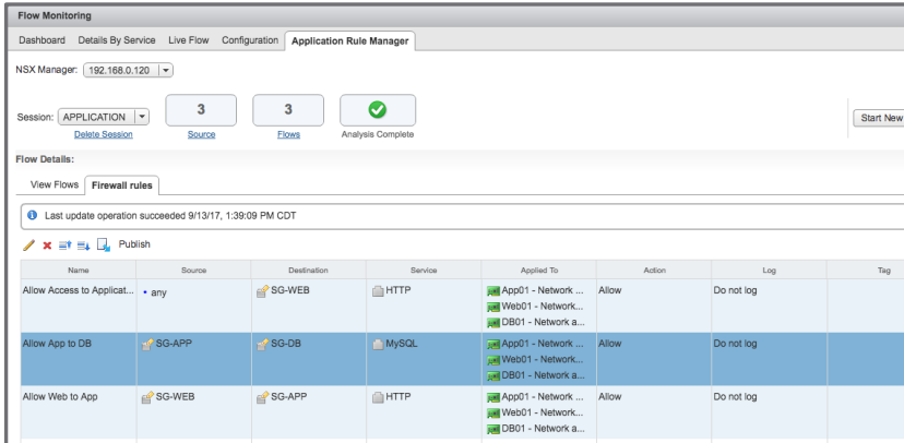
Figure 36 Finish Pre-publish DFW Rules
