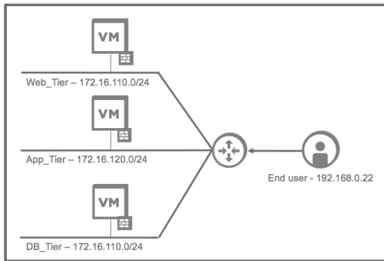
Figure 26 Sample Application Topology
