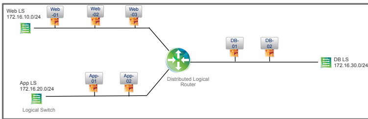
Figure 24 - 3-Tier Application base network topology
