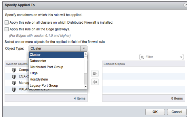
Figure 23 - Applied To scope for the Policy Rule
