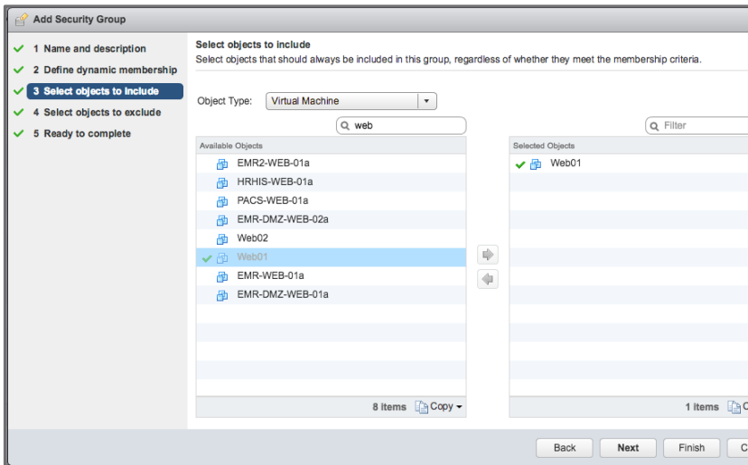
Figure 30 Creating Web NSX Security Group
