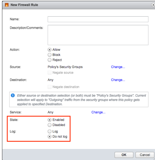
Figure 12 Service Composer Firewall Rule Build
