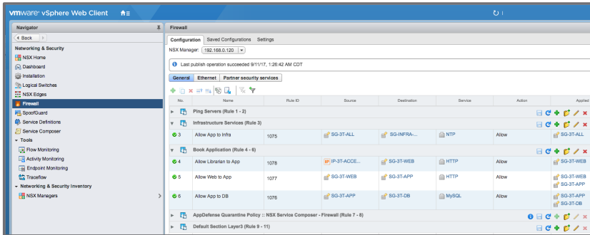
Figure 14 - DFW Policy Rule Table
