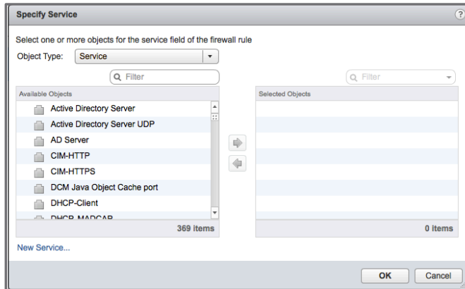
Figure 18 - Source/Destination: Pre-defined Services
