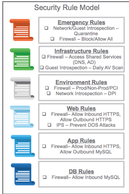
Figure 5 - Security Rule Model
