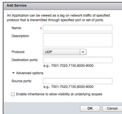
Figure 19 - Source/Destination: Add Custom Services
