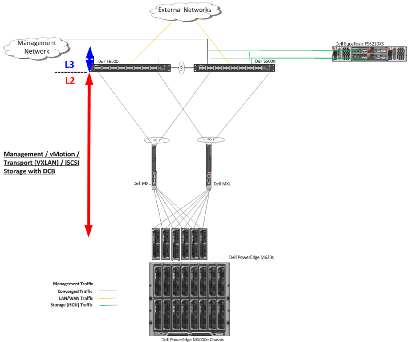
Figure 22: Dell Networking L2 Underlay with iSCSI Storage and DCB
