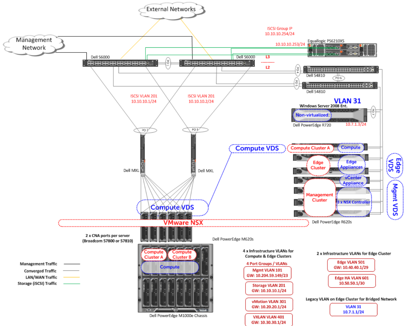
Figure 19: Dell End-to-End Converged Infrastructure with VMware NSX
