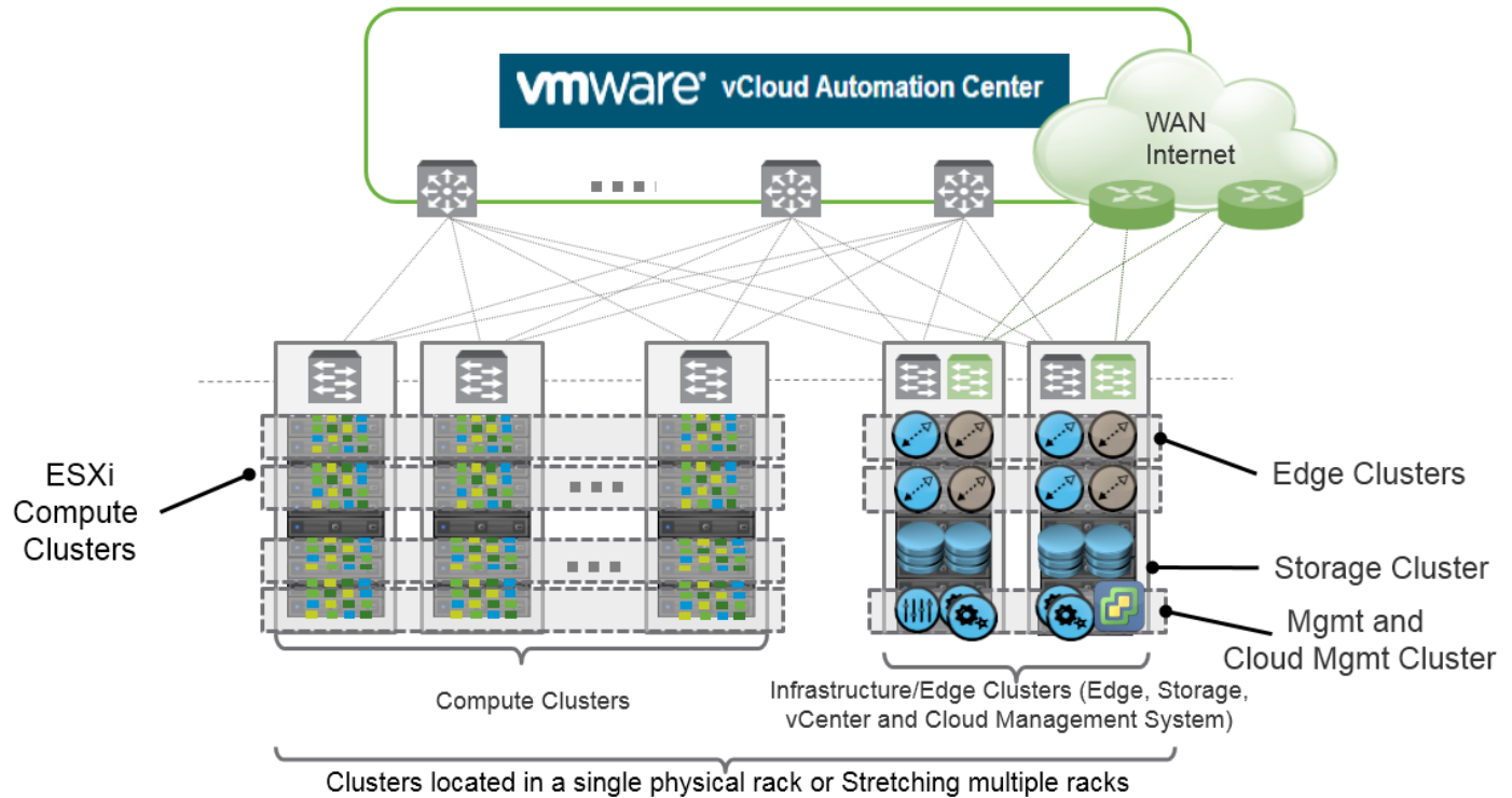
Figure 11: Typical rack layout for compute, management, and edge servers/clusters. Storage can be centrally connected to the core as in a completely converged fabric design or connected to ToR dedicated storage switches at EoR for a typical non-converged design as often shown with Fibre Channel or dedicated iSCSI storage.
