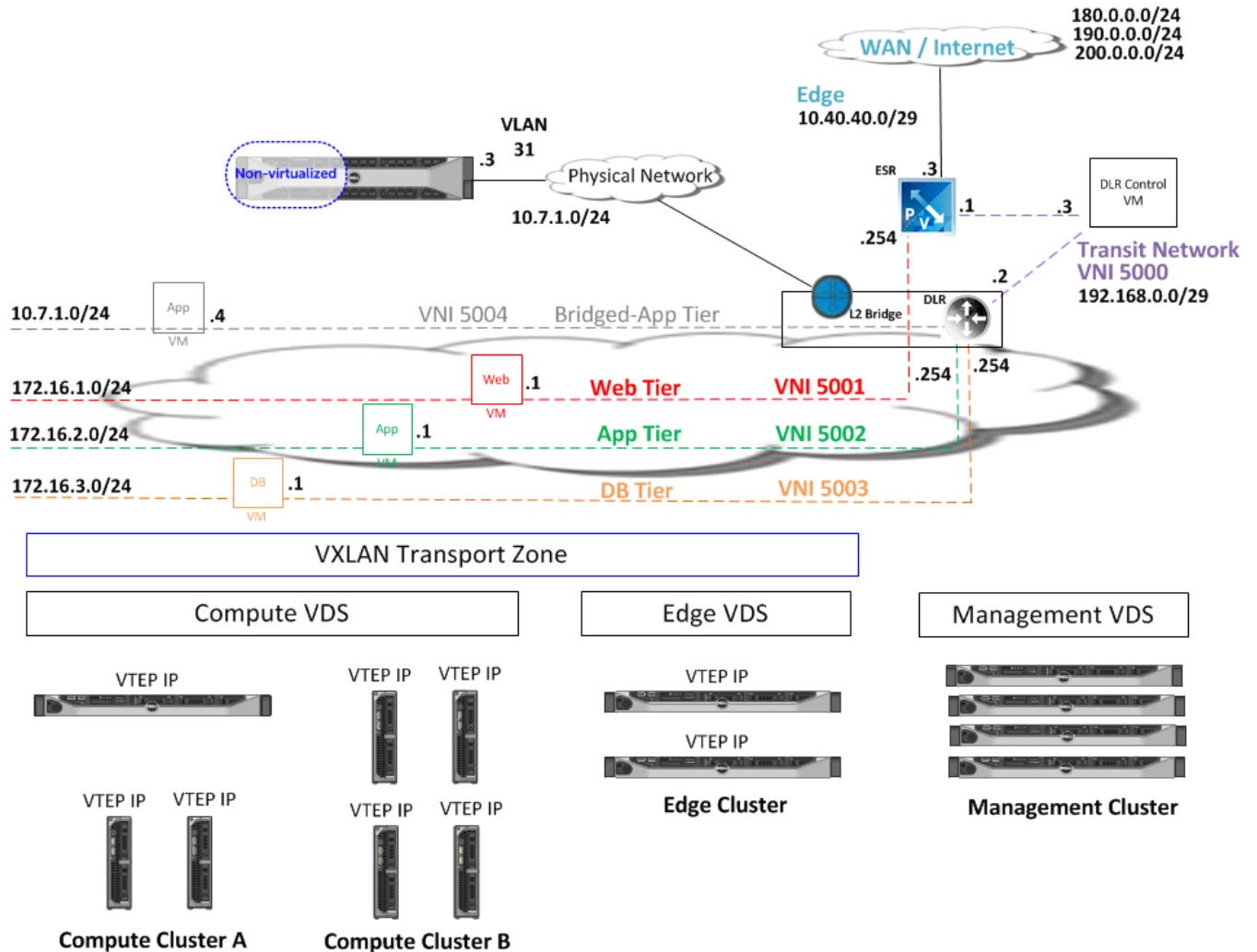
Figure 21: Logical View with the Web Tier logical switch connected to the NSX Perimeter Edge
