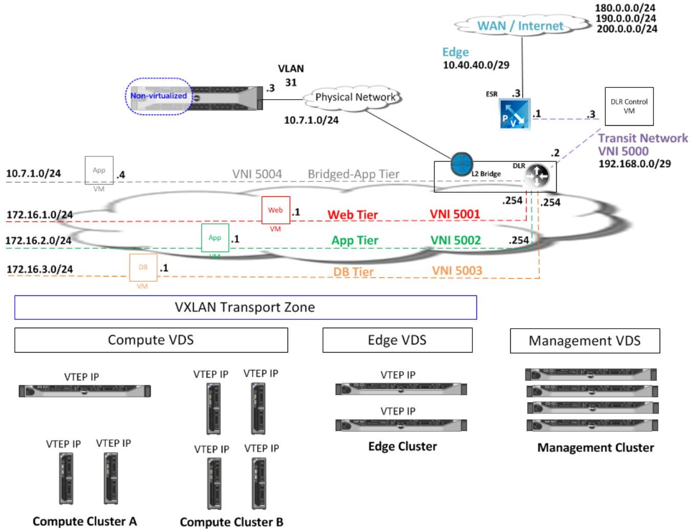
Figure 20: Logical View of Dell End-to-End Converged Infrastructure with VMware NSX
