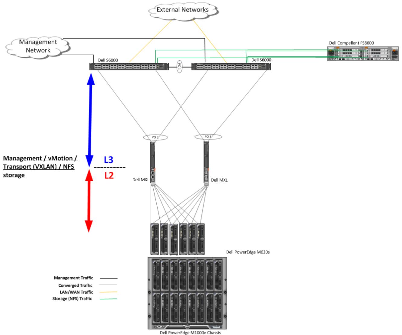
Figure 24: Dell Networking L3 Underlay with NFS Storage
