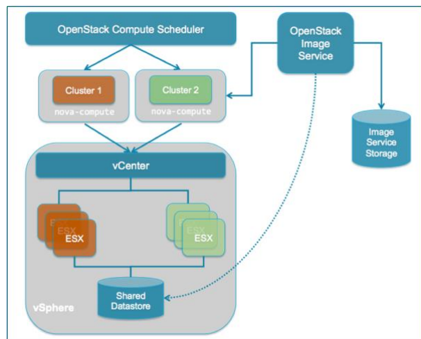
Figure 1.6: OpenStack Image Service
