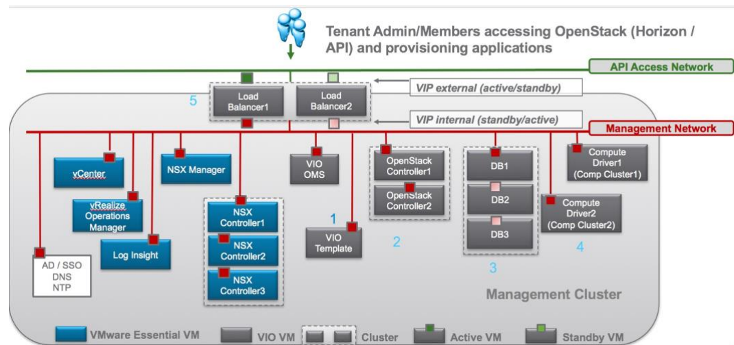
Figure 2.5: VIO Infrastructure deployments
