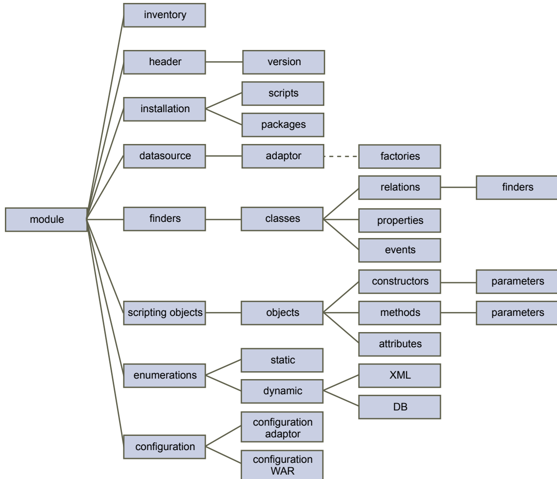
Figure 3-1. Format of the vso.xml Plug-In Definition File
