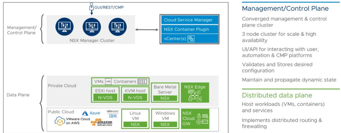
Figure 1 - NSX-T Architecture and Components
