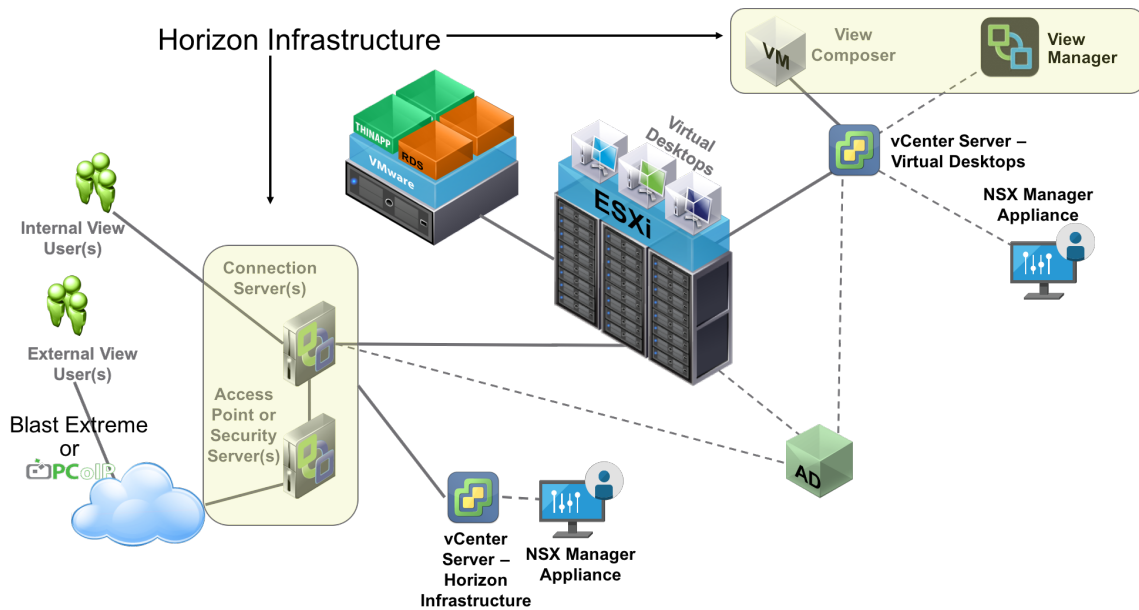
Figure 3: Deployment Topology - Logical
