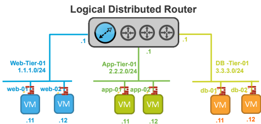
Figure 7 - Micro-segmentation with NSX DFW – Multiple Layer-2 Segment
