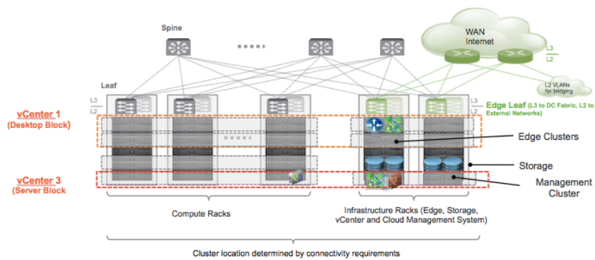
Figure 5b: Deployment Topology with NSX – Physical
