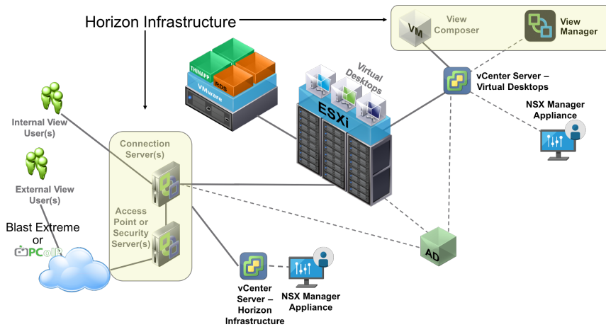
Figure 3: Deployment Topology - Logical
