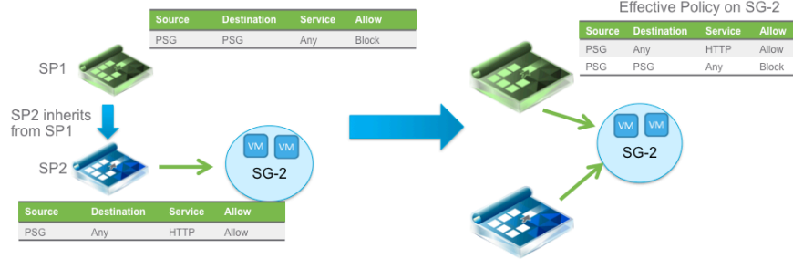
Figure 18 – Rule Inheritance
