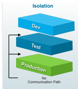
Figure 3 – Network Isolation
