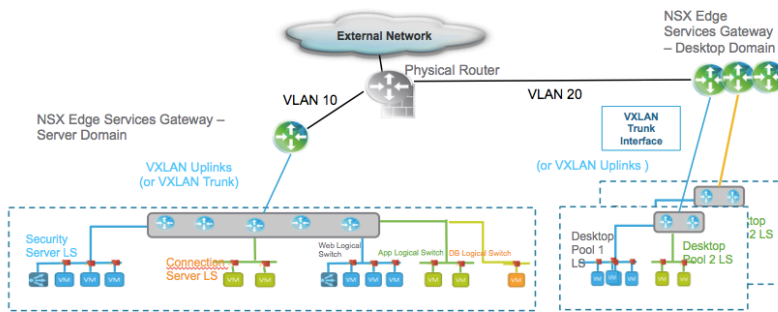
Figure 6: Deploying Horizon with NSX Overlays – Logical Topology
