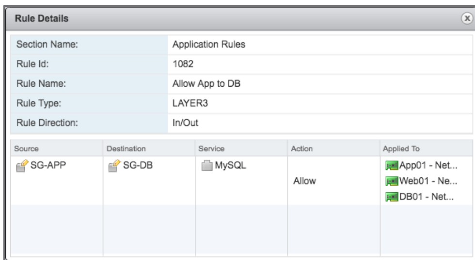
Figure 40 RuleID DFW Details
