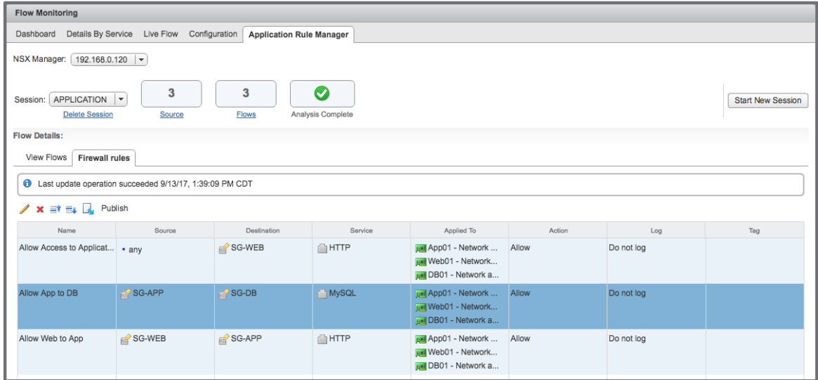
Figure 35 Finish Pre-publish DFW Rules
