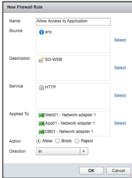
Figure 34 Creating New Firewall Rule
