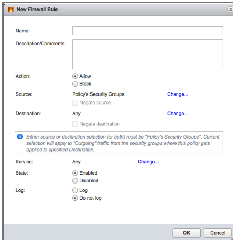
Figure 9 - Service Composer - New Firewall Rule
