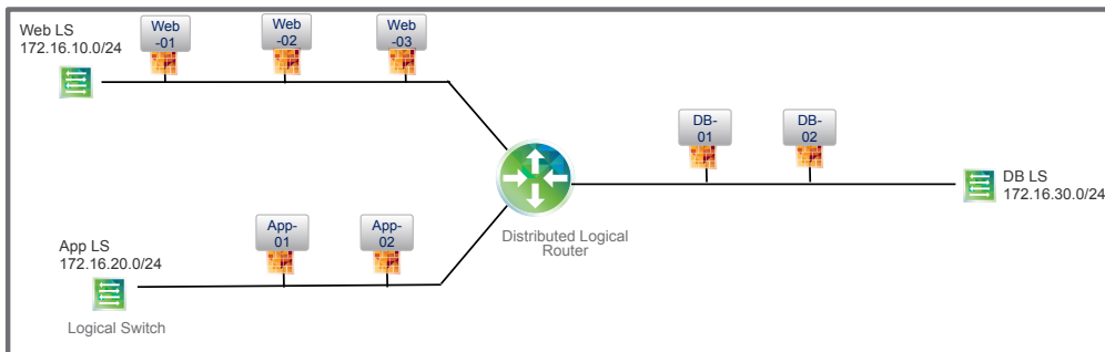
Figure 24 - 3-Tier Application base network topology
