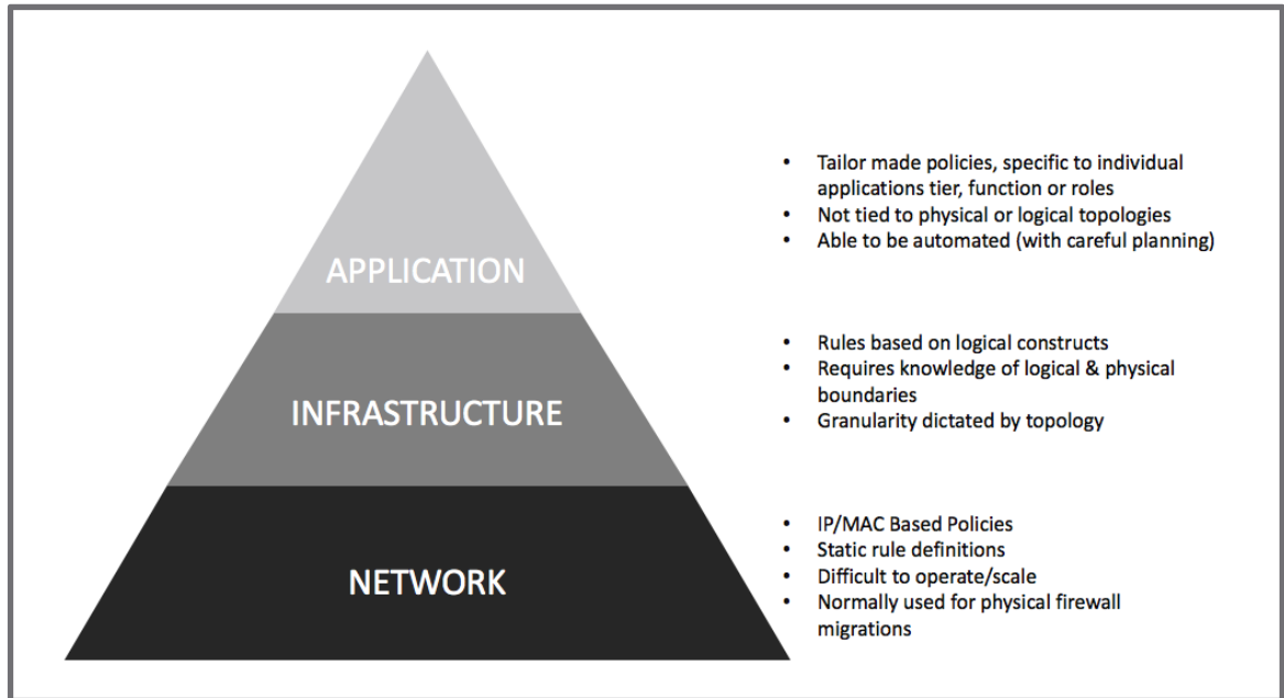
Figure 1 - Micro-segmentation Methodologies
