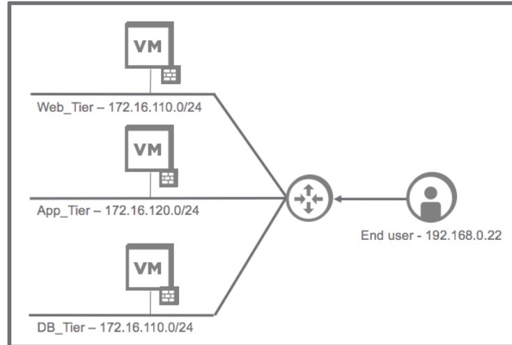
Figure 25 Sample Application Topology
