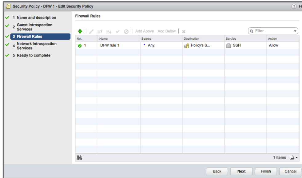
Figure 4 - NSX Security Policy Interface
