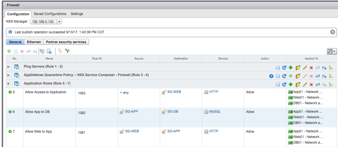
Figure 37 New Rules placed into DFW Interface
