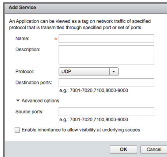
Figure 19 - Source/Destination: Add Custom Services
