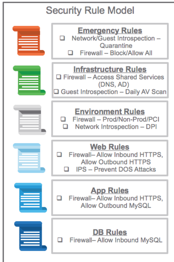
Figure 5 - Security Rule Model
