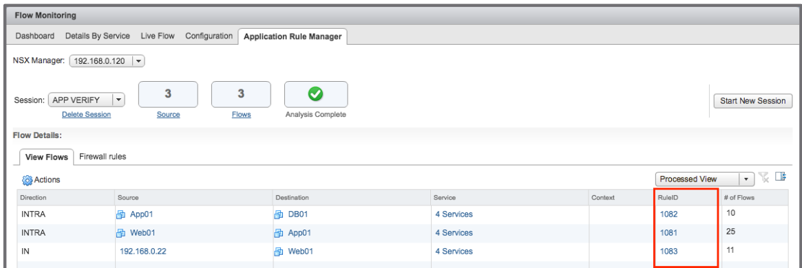
Figure 39 Verify Monitor Session with new RuleID entries
