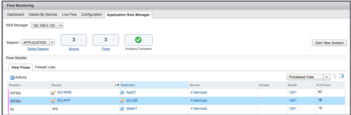
Figure 30 Source Groups Resolved
