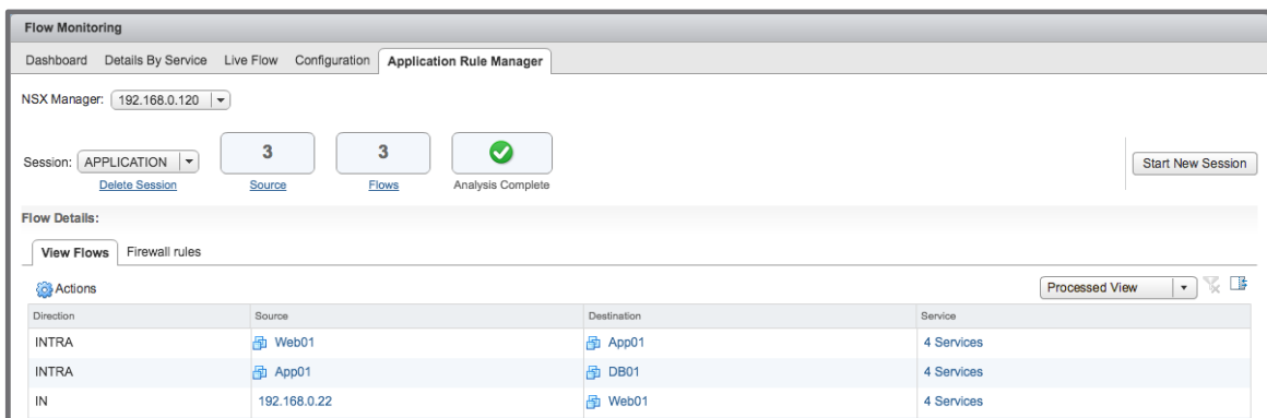
Figure 28 ARM Completed and Analyzed Monitor Session
