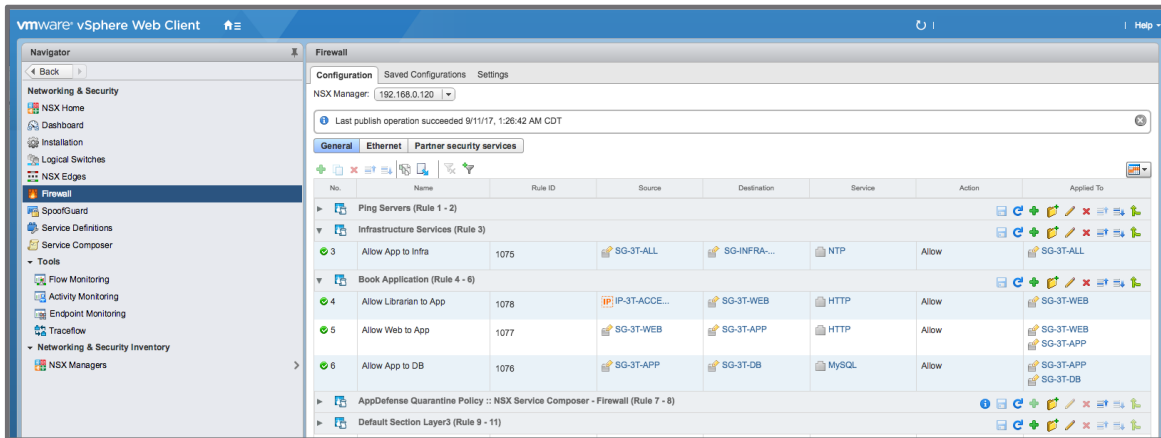
Figure 14 - DFW Policy Rule Table
