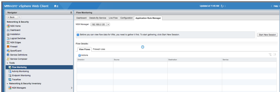
Figure 26 Application Rule Manager interface
