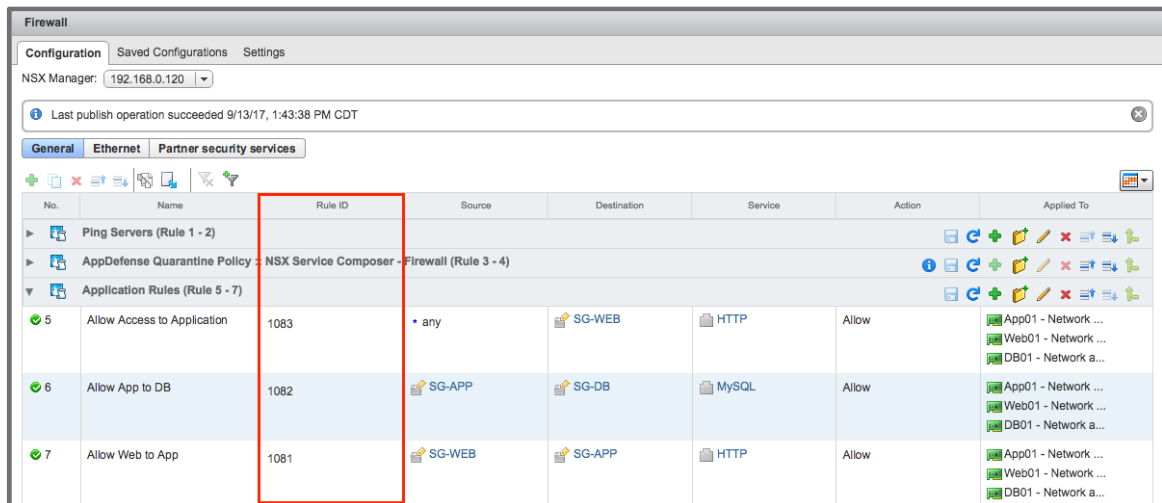
Figure 38 New RuleIDs for New Rules
