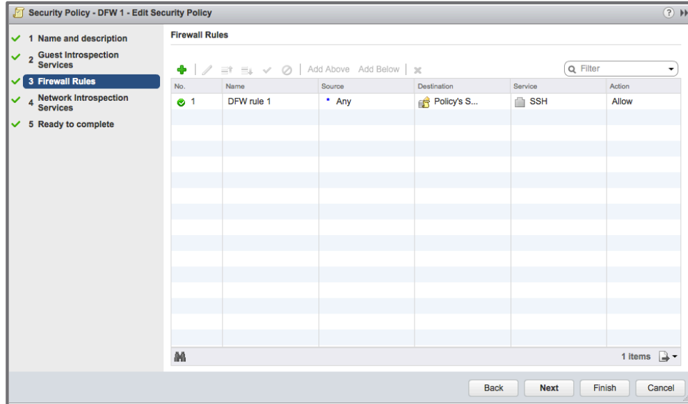
Figure 8 – Service Composer - Security Policy Creation
