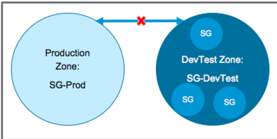
Figure 13 - Prod - Non-Prod Restriction
