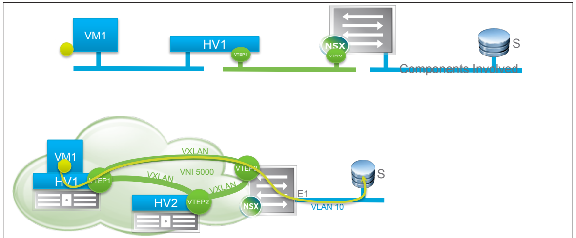
Figure 9: Unicast traffic from VM1 to server S
