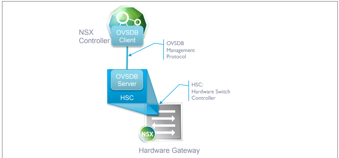
Figure 8: Connection Hardware Gateway/NSX Controller
