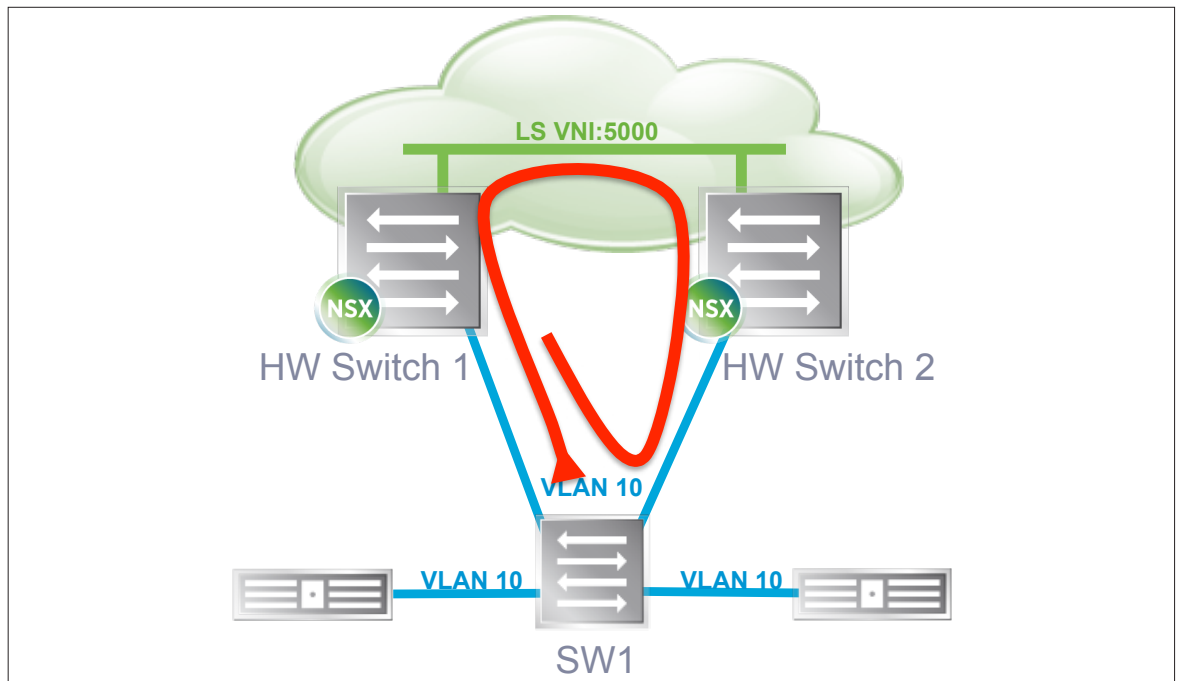
Figure 14: Loop between Hardware Gateways resulting from a cabling error
