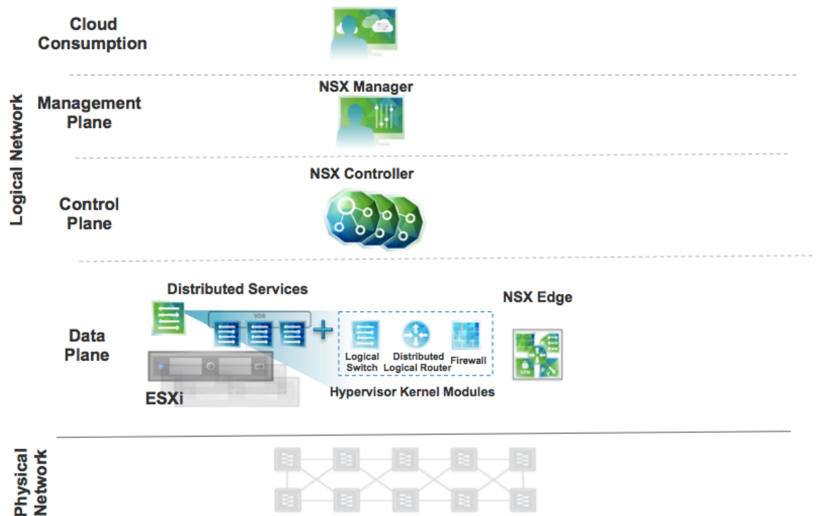
Figure 1 - VMware Network Virtualization Solution Components
