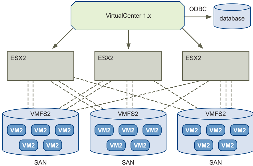
Figure 3-2. Typical Environment Before HVL Alignment
