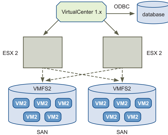
Figure 3-1. Typical Environment for In-Place Upgrade
