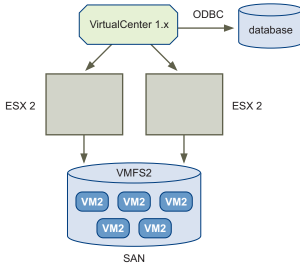
Figure 3-4. Typical Environment for Upgrading Hosts on a SAN Using Upgrade VMotion
