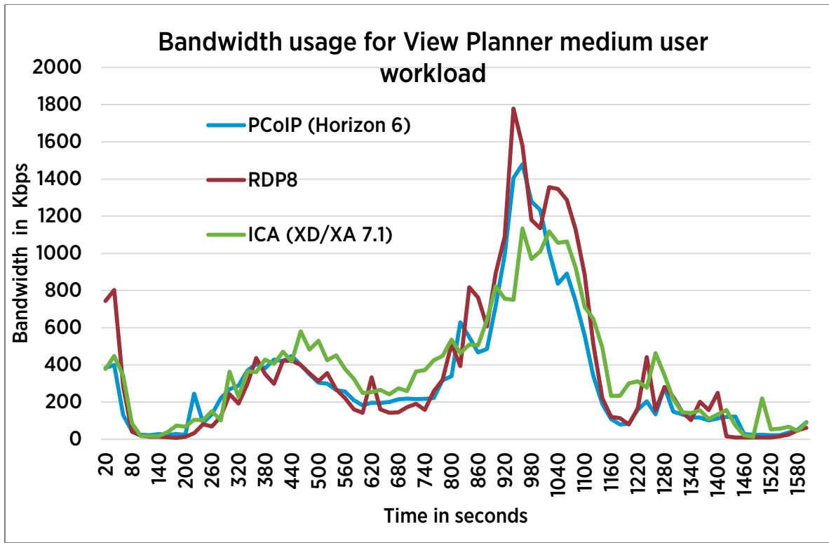
Figure 11. Bandwidth usage for View Planner medium user workload for three competing remote display protocols
