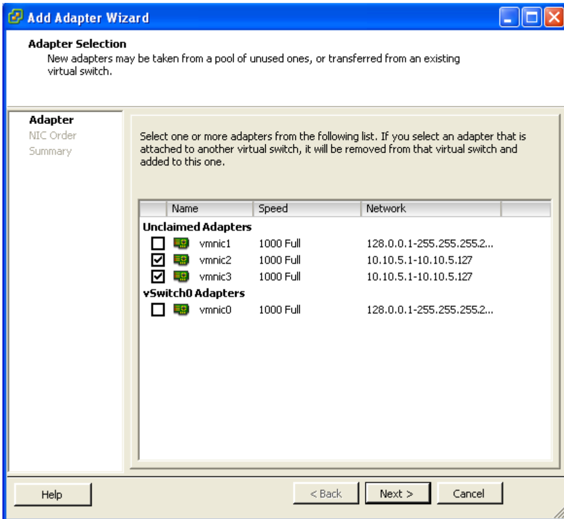
Figure 6: vCenter GUI - Add Adapter Wizard
