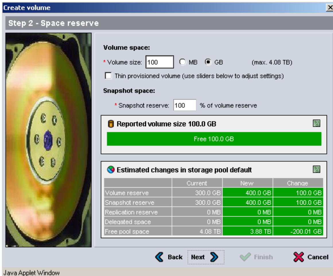
Figure 12: Group Manager GUI - Create Volume – Space Allocation
