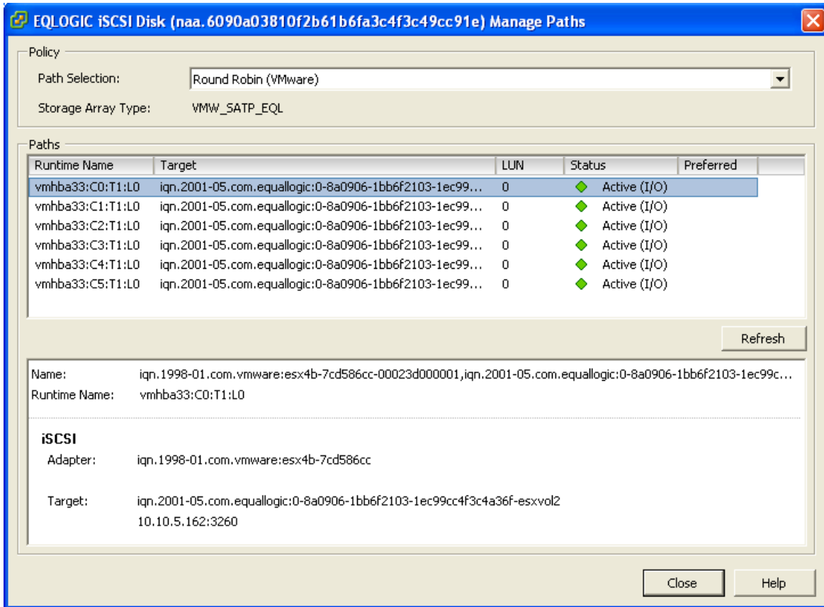
Figure 16: vCenter GUI - Round Robin MPIO Policy for New Volume
