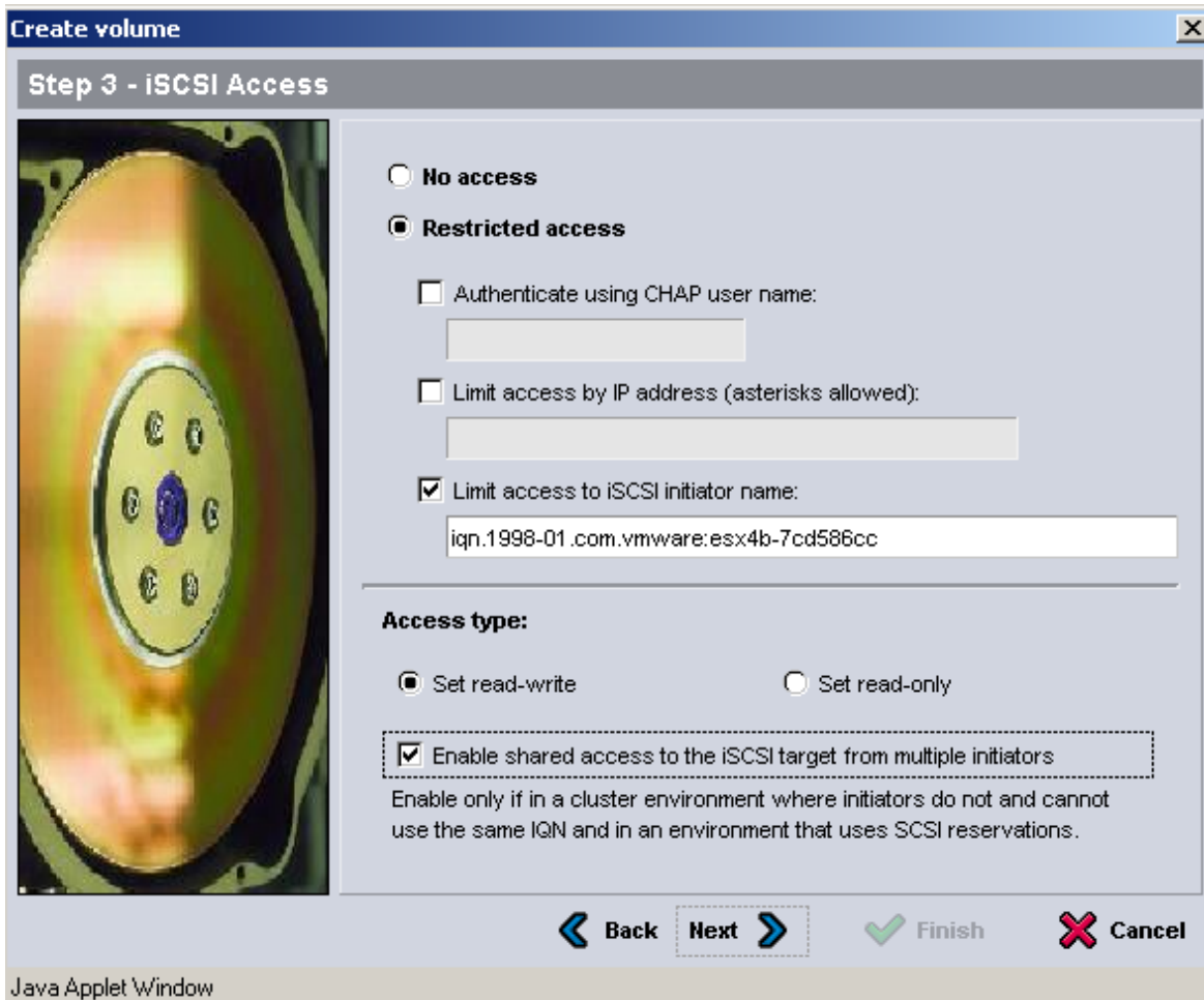
Figure 14: Group Manager GUI - Create Volume – iSCSI Access Control
