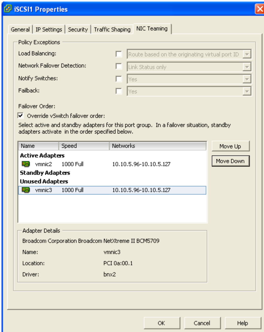
Figure 7: vCenter GUI - Mapping VMkernel Ports to vmnics
