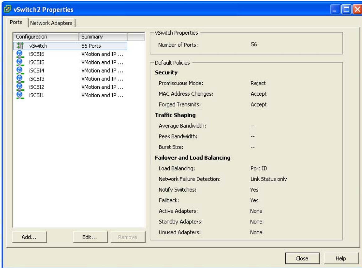
Figure 5: vCenter GUI - vSwitch Properties
