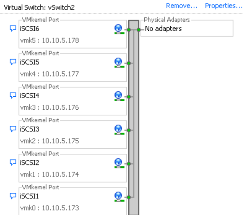
Figure 4: vCenter GUI - VMkernel Ports
