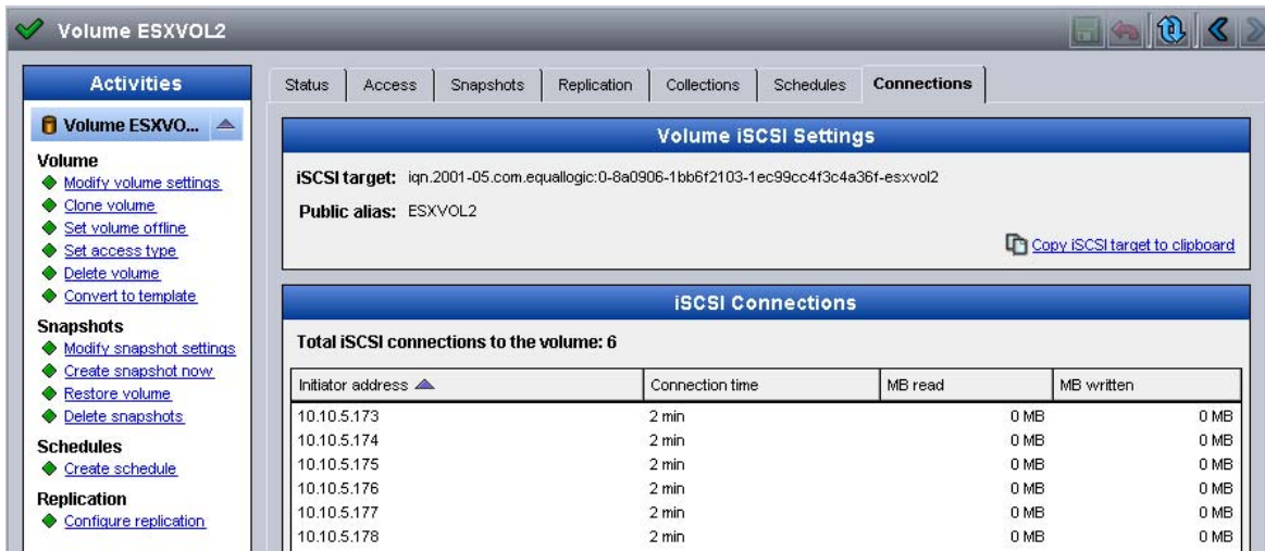
Figure 17: Group Manager GUI - Multiple Connections in Group Manager
