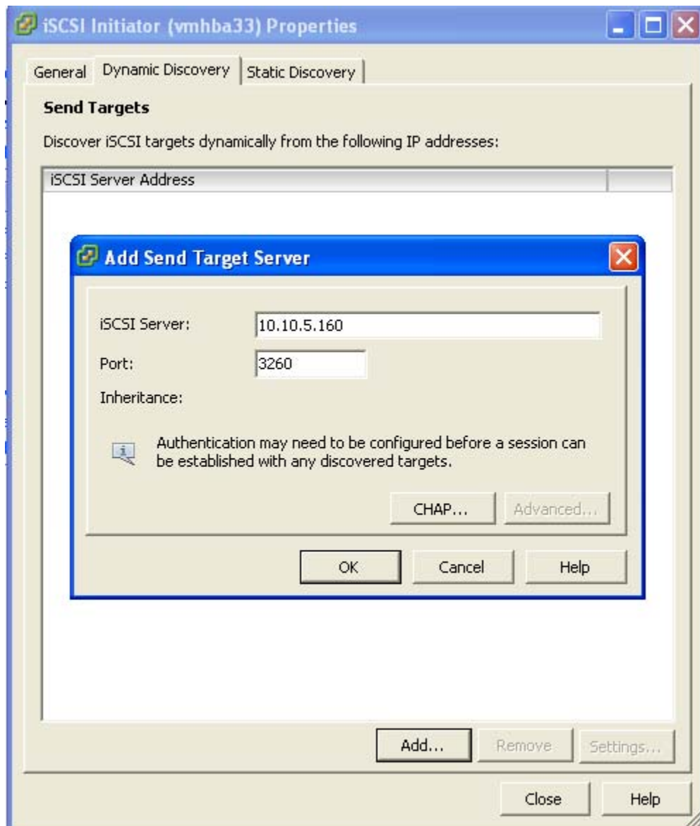
Figure 10: vCenter GUI - Add Group IP Address to Dynamic Discovery
