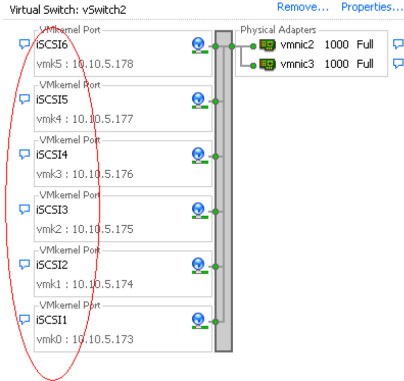
Figure 9: vCenter GUI - Noting the vmk# of the VMkernel Ports
